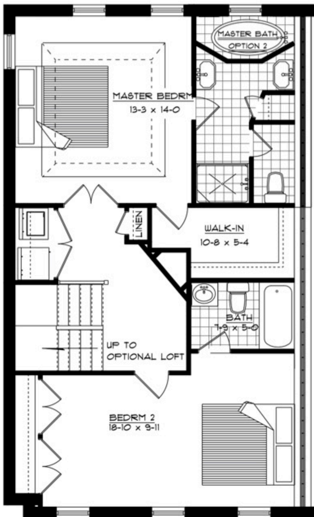
THIRD FLOOR
